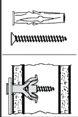
Nylon winged Wall plug
