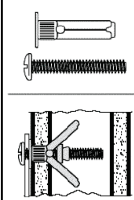
TASSELLO "MOLLY"
